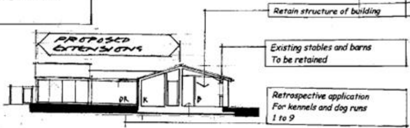
PROPOSED END ELEVATION SOUTH WEST 1:200
