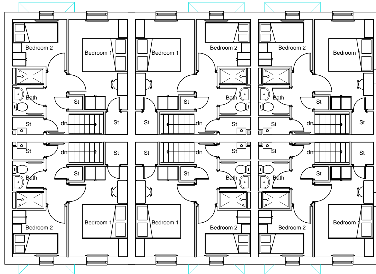
FIRST FLOOR PLAN Type Acomb (end/mid)
