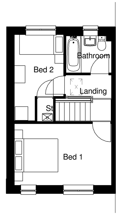
First Floor. 1 : 100
