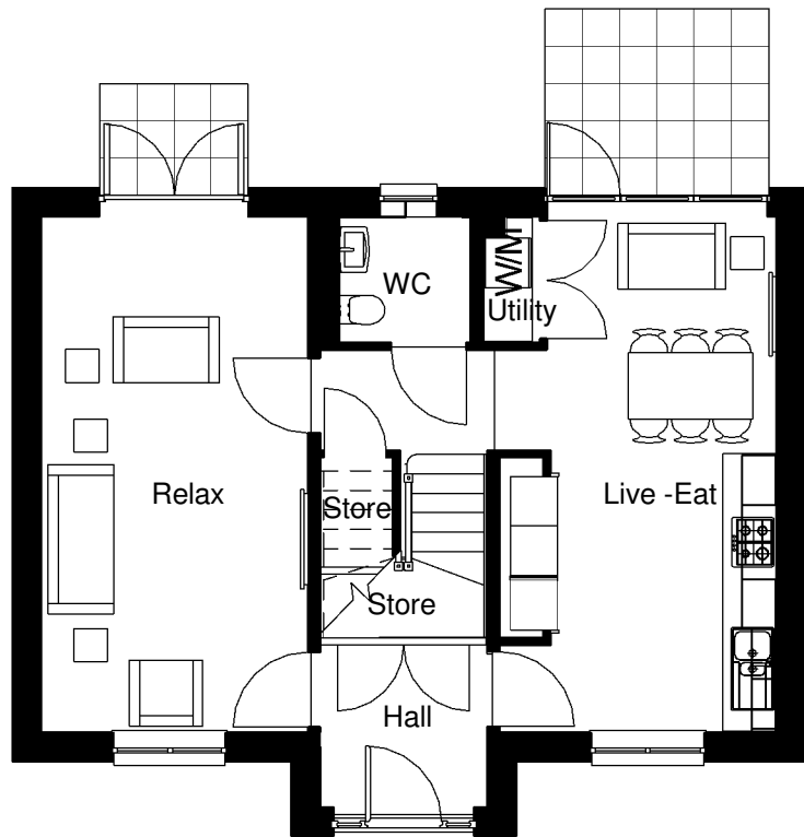
Ground Floor. 1 : 100
