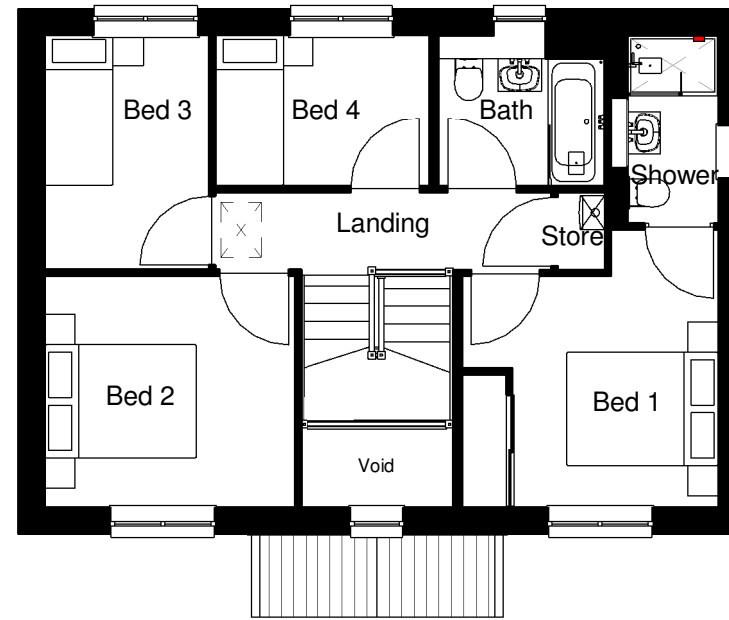
First Floor. 1 : 100
