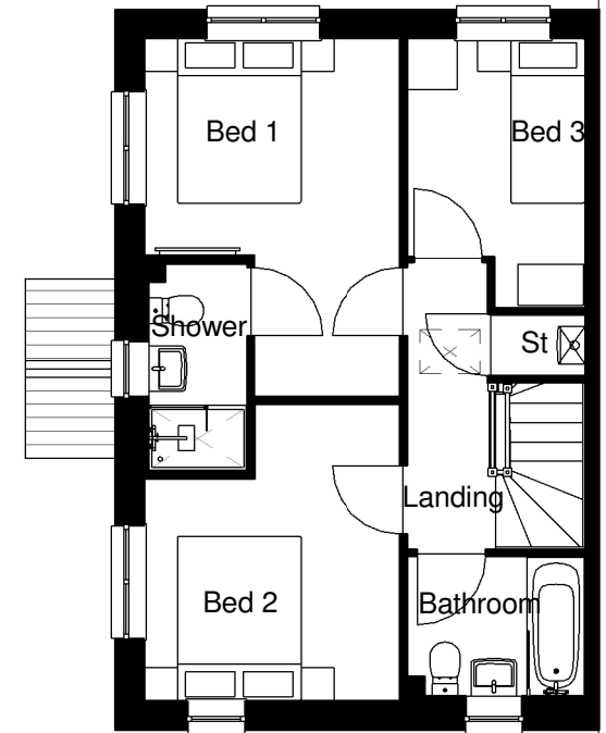
First Floor. 1 : 100
