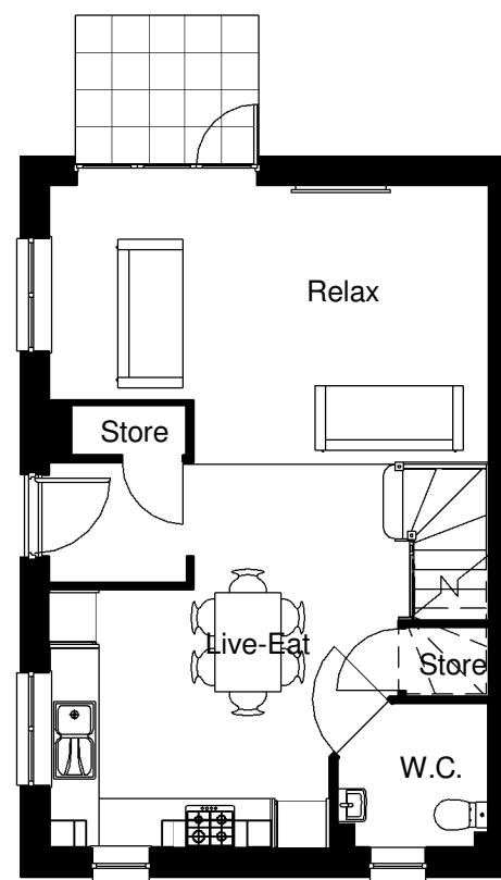
Ground Floor. 1 : 100
